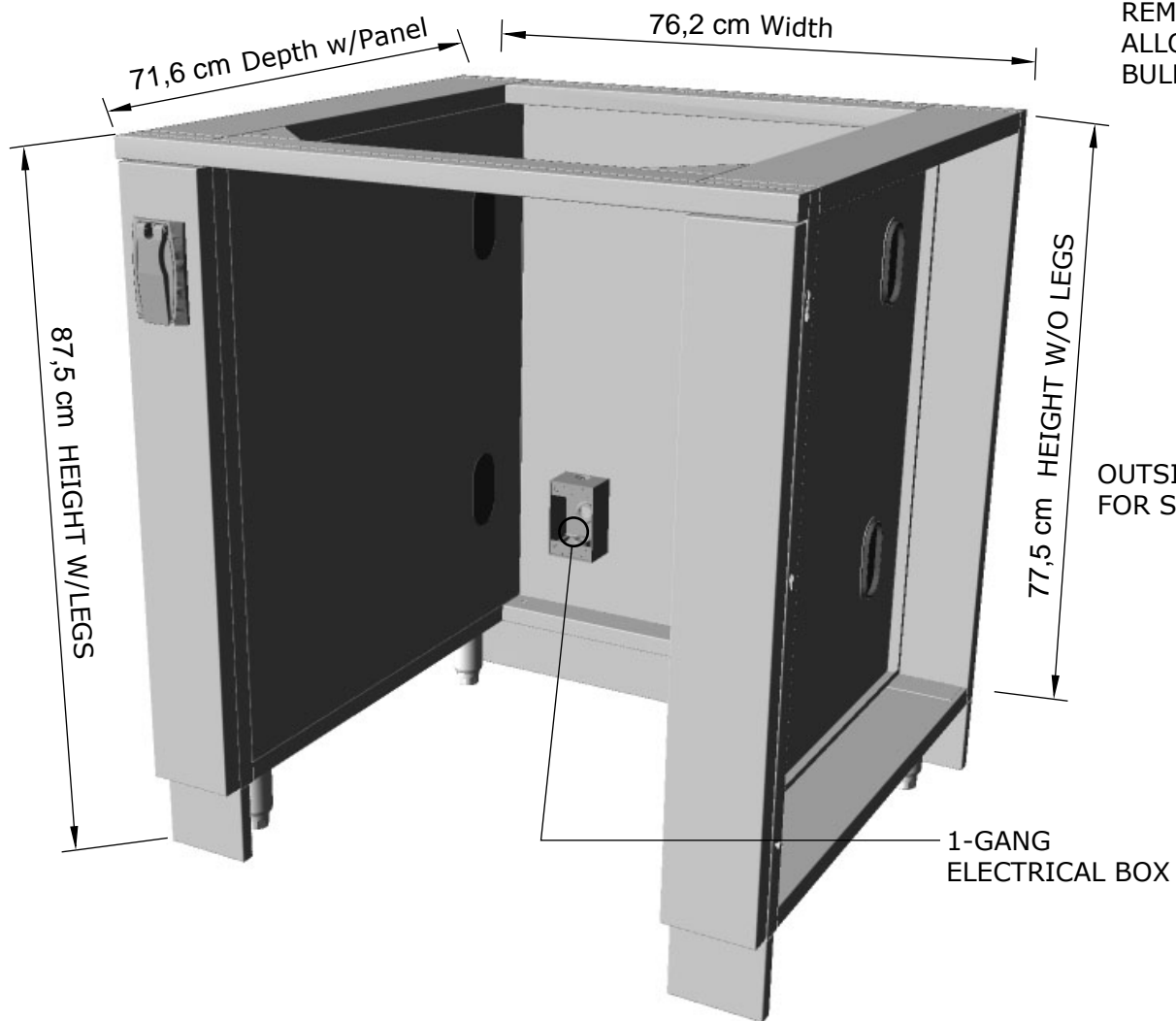
ISO VIEW
