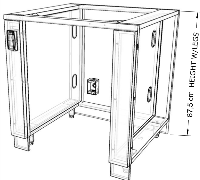
ISO VIEW
